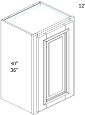
Single Door Wall Cabinet
