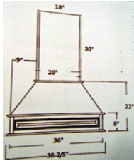
CWH36: Wood Hood
